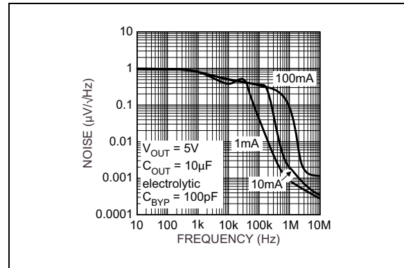
FIGURE 2-16: Noise Performance.
