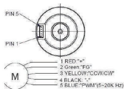
Brushless motor wiring diagram
