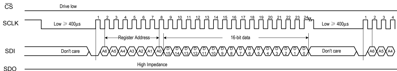
Figure-6 Write Sequence in Three-Wire Mode
